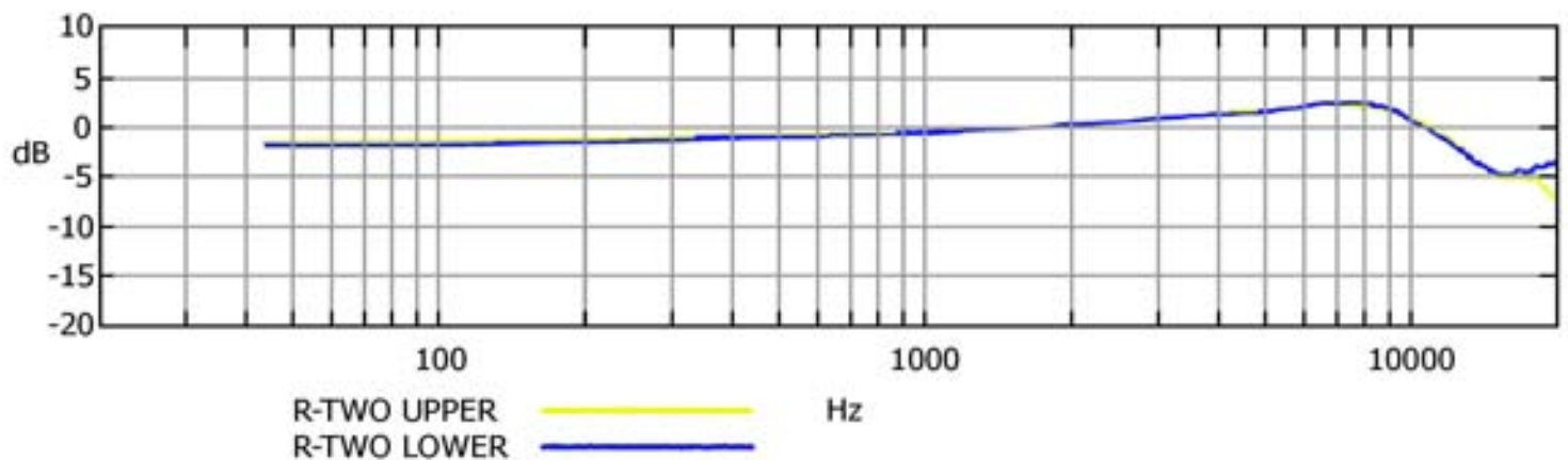
R-TWO FREQUENCY RESPONSE
